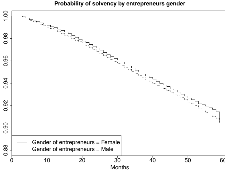
Figure 1: Kaplan Meier curves of the probability of solvency by entrepreneurs gender
